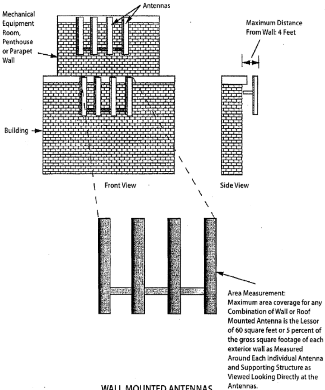
WALL MOUNTED ANTENNAS
